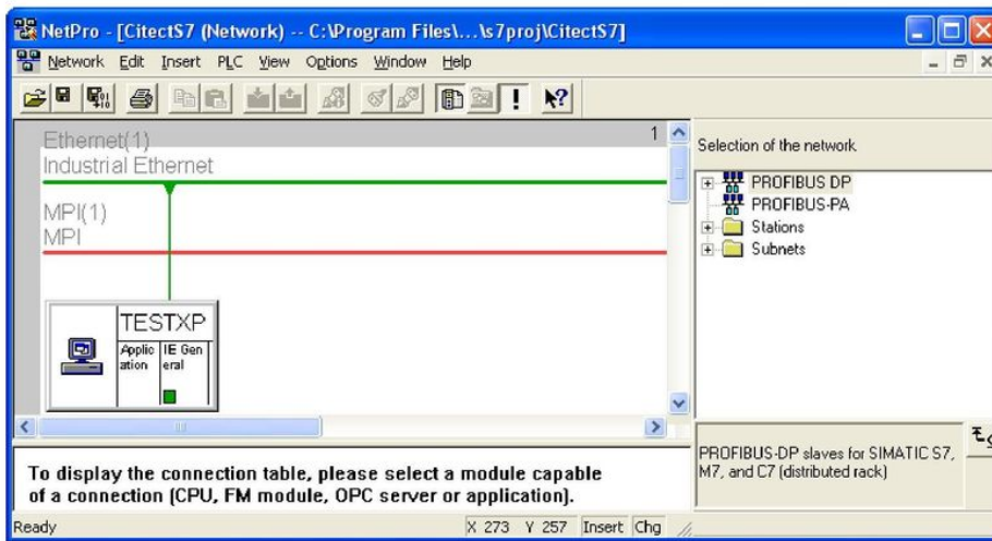
Fig. 24: NetPro configuration
